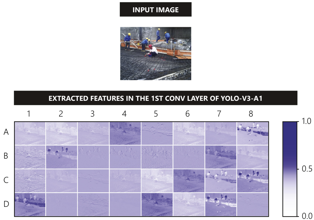
Fig. 13. Example of extracted features in the first convolutional layer of YOLO-v3-A1 model.
