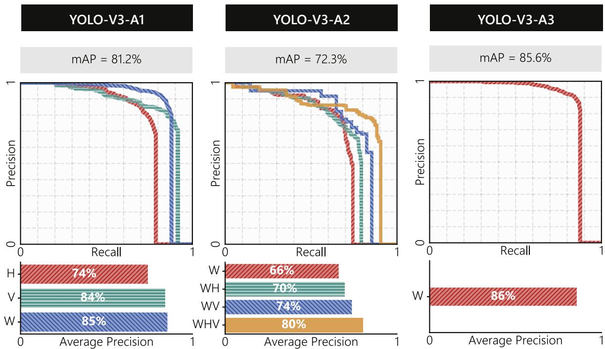
Fig. 14. Performance of the YOLO-v3 models in three approaches.
