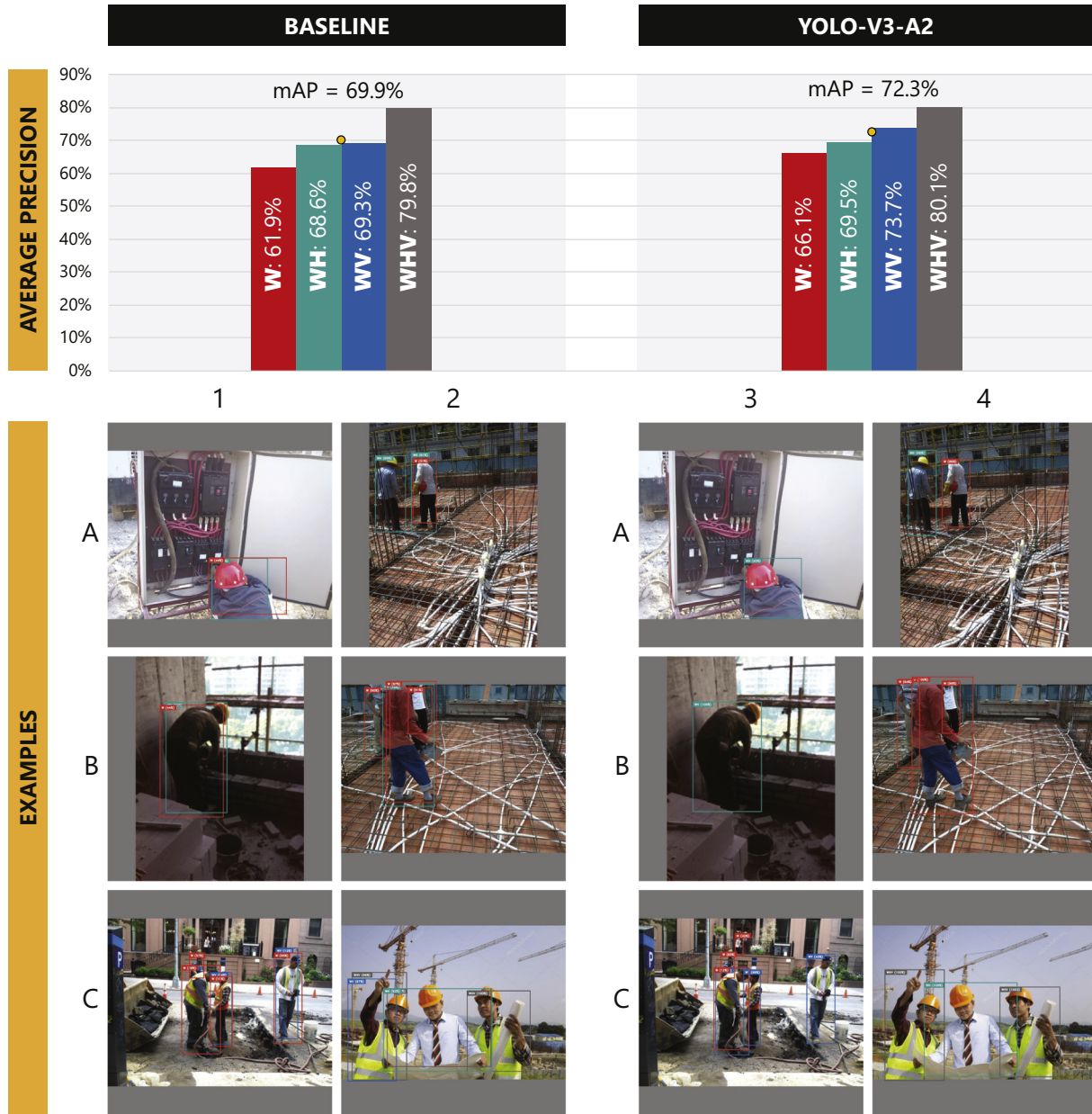
Fig. 17. Comparison between baseline YOLO-v3 model and modified YOLO-v3-A2 model in Approach-2.
