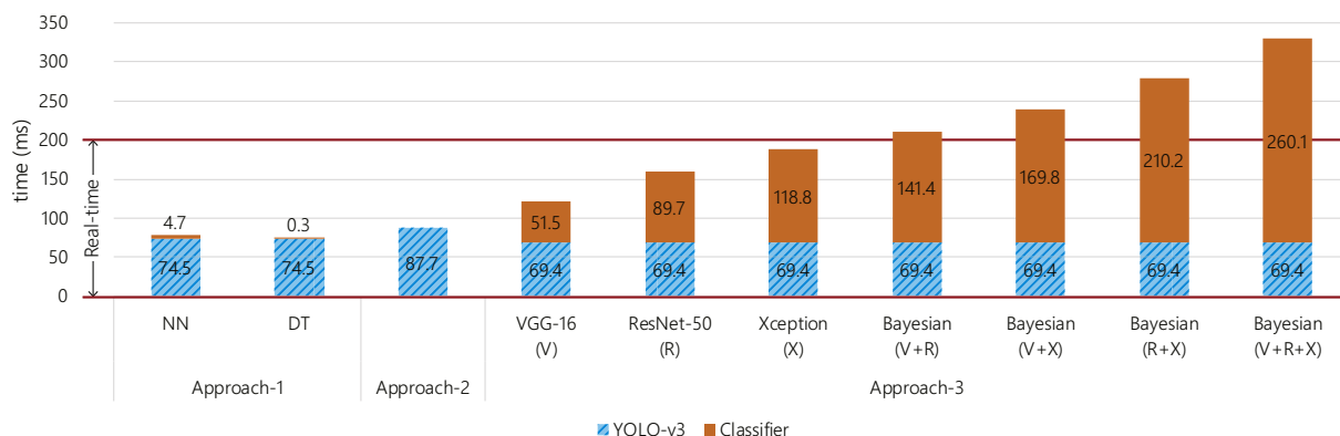
Fig. 20. Average time for processing one test image in each approach.
